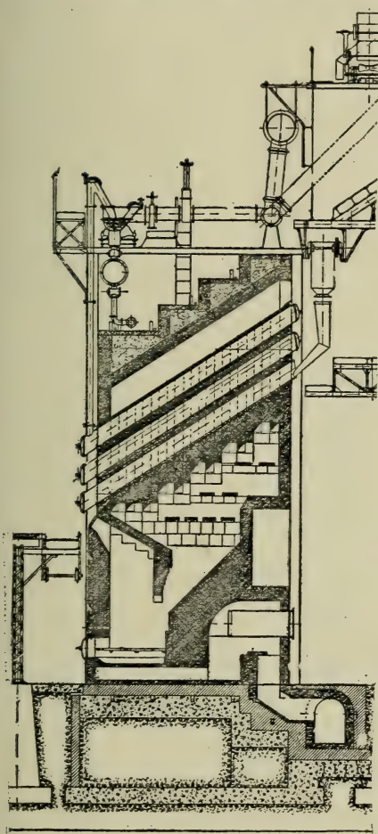
FIG. 87.—Inclined Gas-Works Retort.
